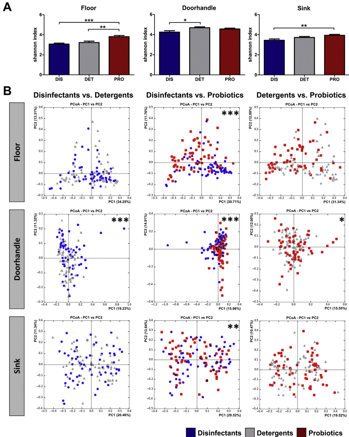
Fig. 2. Diversity metrics of the environmental microbiota upon different sanitization strategies. (A) Alpha diversity of each environmental site after different sanitization using strategies. Shown is the Shannon index (mean \pm standard error of the mean, * p < 0.05; ** p < 0.01; *** p < 0.001, ANOVA). (B) Principal coordinates analysis of the beta diversity using weighted Unifrac distances. Shown are pairwise comparisons between different sanitization strategies. Statistical significance was calculated by PerMANOVA (* p < 0.05; ** p < 0.01; *** p < 0.001).
